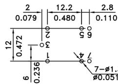
Installation size diagram(bottom view) The wiring diagram(bottom view)
