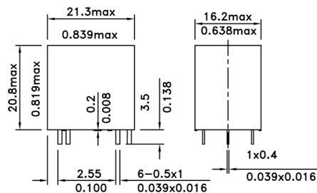
Outline Dimension
