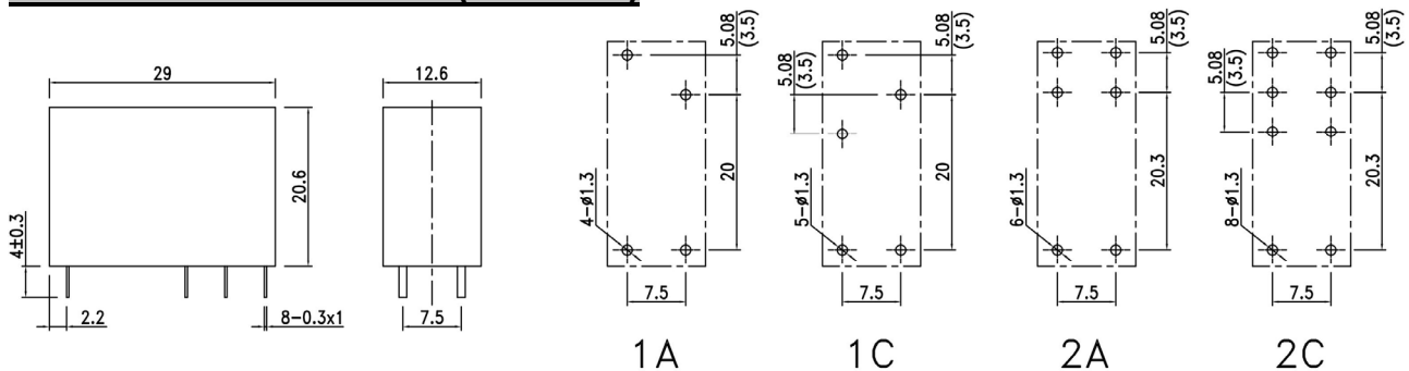
Outline Dimension
